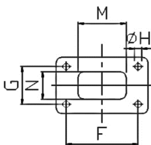
View from "W" (Flange Details)
